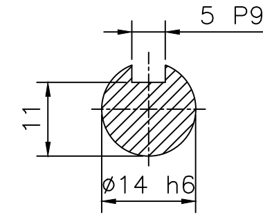
INPUT & OUTPUT SHAFT KEYWAY
